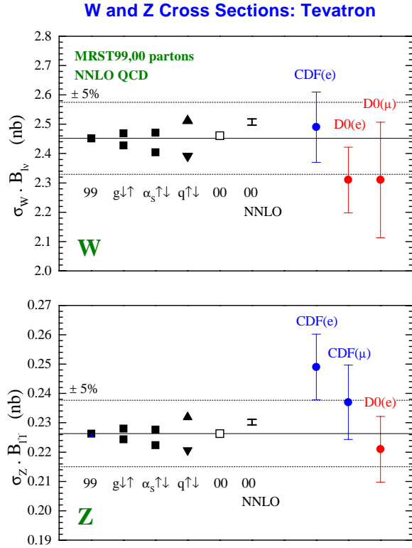
Fig. 5. The solid squares and triangles are the predictions of the NLO' cross sections of (23) for W and Z production and leptonic decay in p\bar{p} collisions at \sqrt{s} = 1.8 TeV obtained using various NLO sets of MRST99 partons [25]. The open square and small error bar are, respectively, the NLO and NNLO predictions of (22) using the MRST00 partons [26]. Also shown are the experimental measurements from CDF [29] and D0 [30]. For ease of reference \pm 5\% lines are shown about the MRST99 default prediction. We thank W.J. Stirling for this figure, which combines results presented in [25,26]
