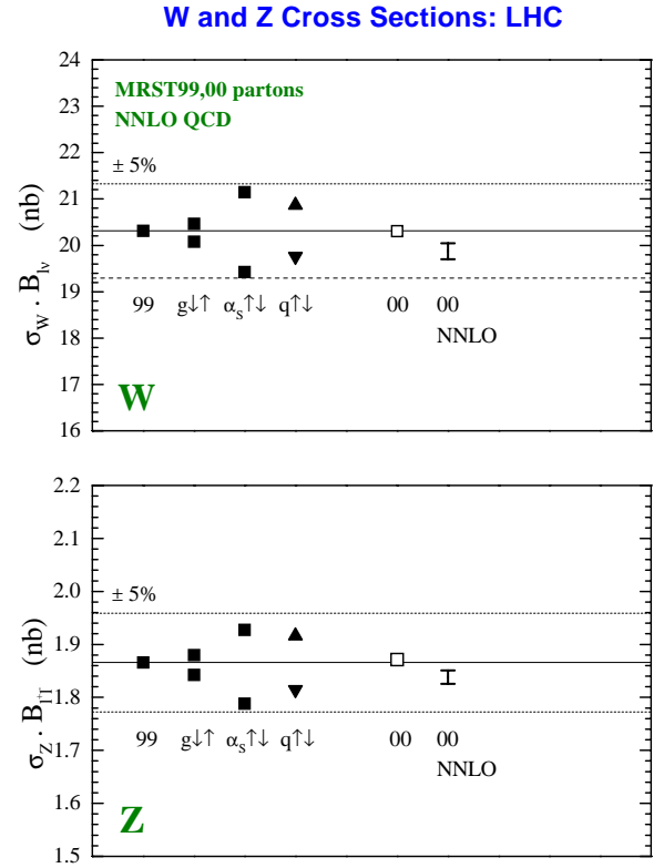
Fig. 6. As for Fig. 5 but for pp collisions at \sqrt{s} = 14 TeV
