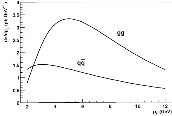
Fig. 8. Contributions to the diphoton p_t spectrum from the diagrams of Fig. 7 in pp collisions at \sqrt{s} = 14 TeV. Each photon is required to have transverse momentum p_{\gamma t} > 20 GeV and rapidity |\eta_\gamma| < 1 . The photons are required not to lie within the same \eta - \phi cone of radius 0.4. We thank M.A. Kimber for this figure
