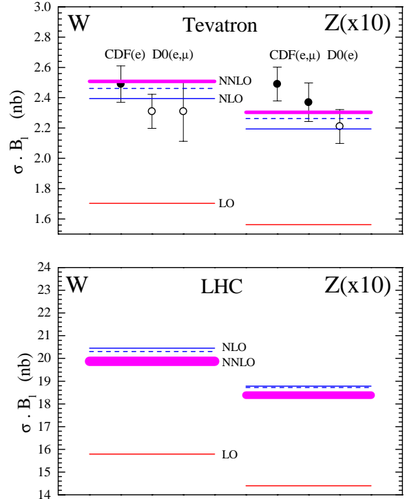
Fig. 4. The predictions of the cross sections for W and Z production and leptonic decay at the Tevatron and the LHC obtained from parton sets of LO, NLO and NNLO global analyses of the same data set [26]. The cross sections labelled LO, NLO and NNLO are as in (22) and the dashed line is the NLO' prediction of (23). The band of the NNLO predictions allow for the ambiguity in the NNLO splitting functions [28]. Also shown are measurements obtained at the Tevatron [29,30]. The figure is taken from [26]
