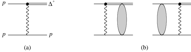
Fig. 1. a \Delta^+ production mediated by photon exchange, and b possible rescattering corrections
