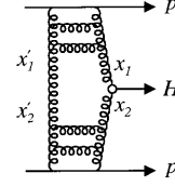
Fig. 9. Higgs production via Pomeron-Pomeron fusion in pp collisions
