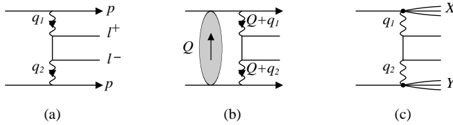
Fig. 3. a Lepton pair production in pp collisions, b one of the rescattering corrections, and c a possible contamination coming from proton dissociation into X, Y systems
