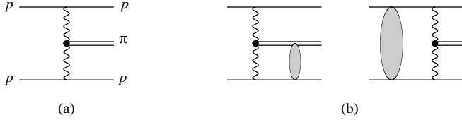
Fig. 2. a \pi^0 production mediated by photon exchanges and b two of the possible rescattering corrections
